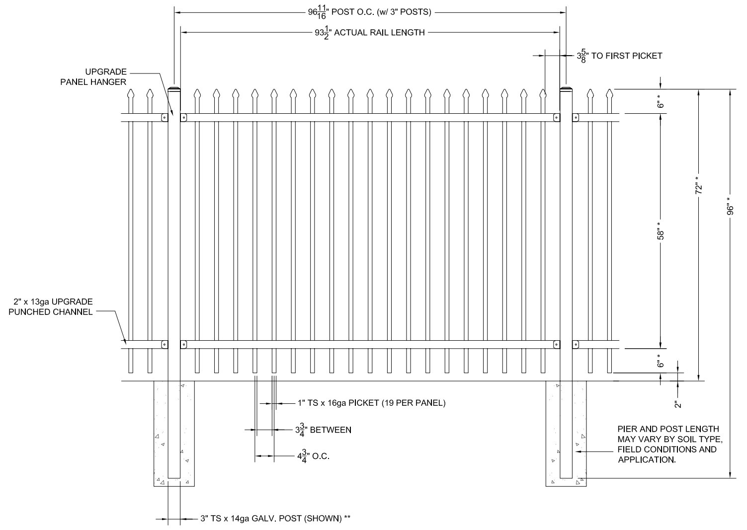
1 TYPICAL ELEVATION SCALE: NTS
