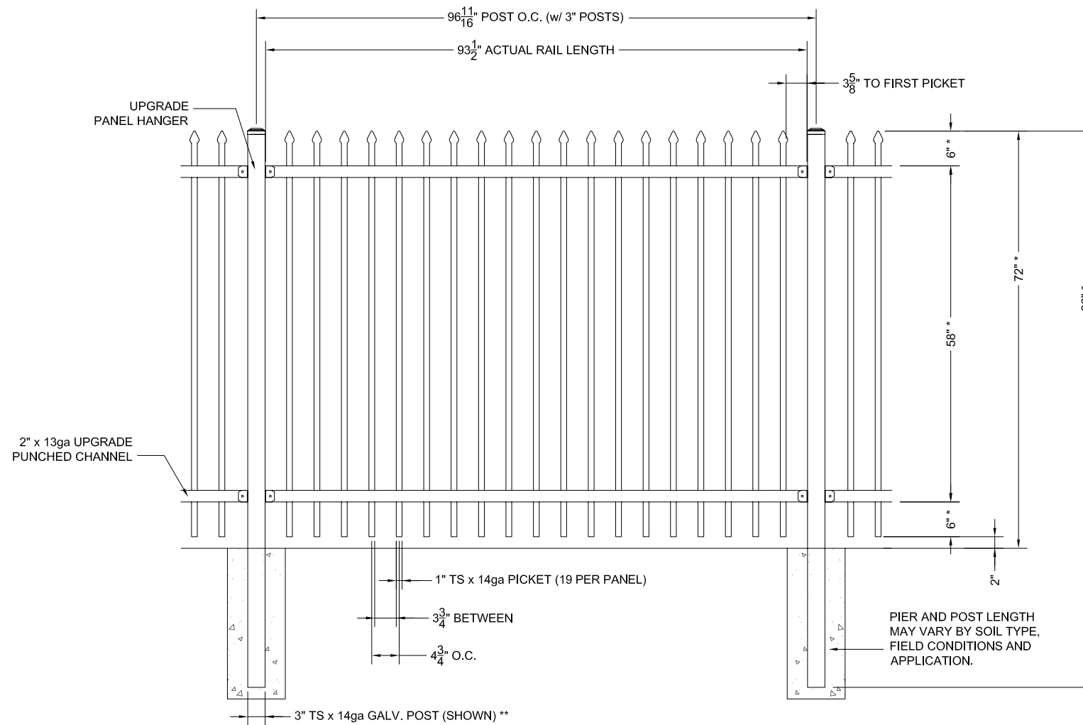
1 TYPICAL ELEVATION SCALE: NTS
