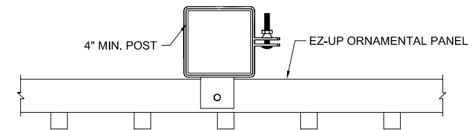
1 LINE POST DETAIL SCALE: NTS
