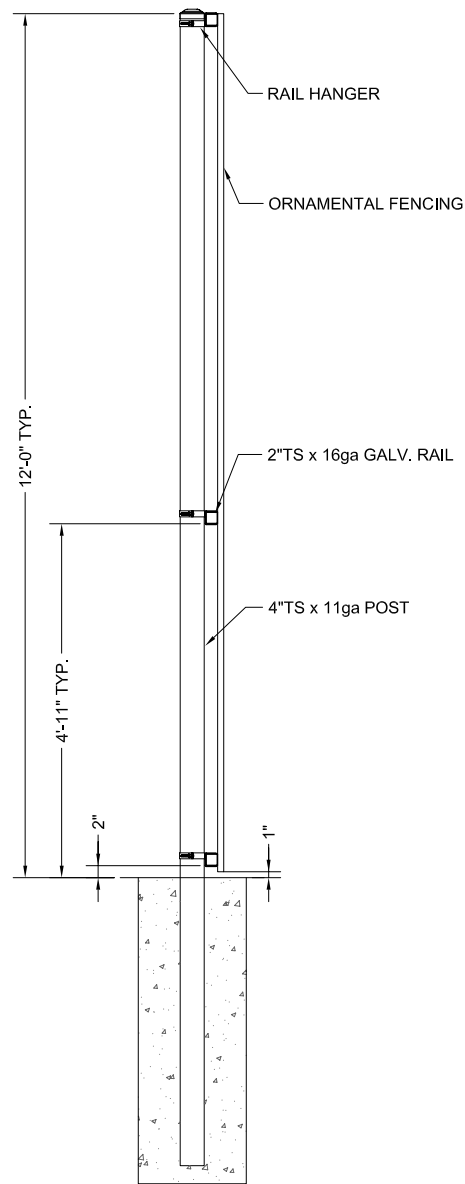
A EZ-UP ORNAMENTAL SECTION SCALE: NTS
