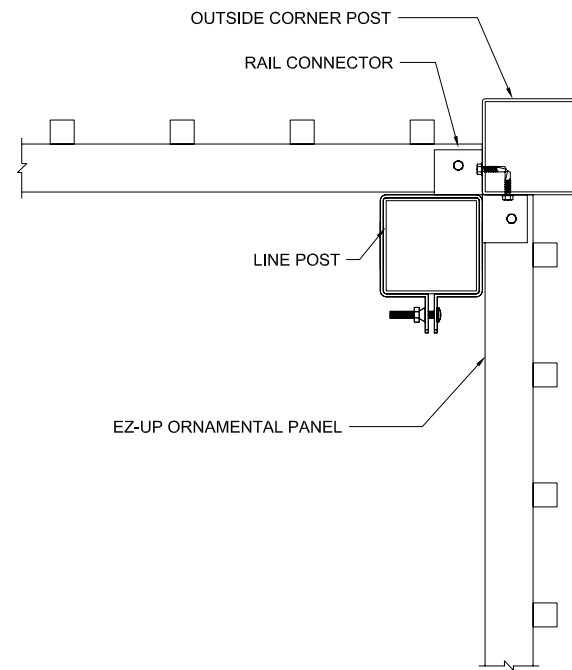
4 OUTSIDE CORNER DETAIL SCALE: NTS
