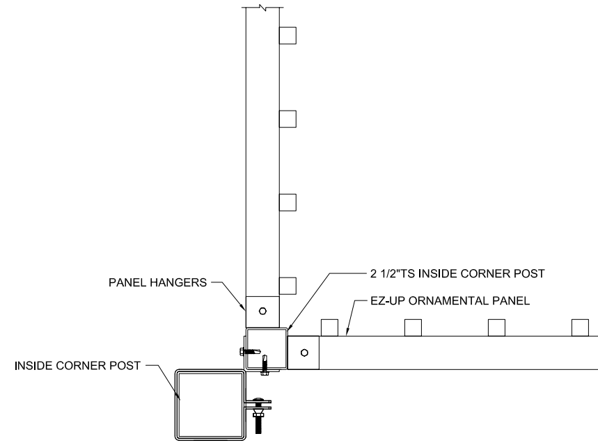
2 INSIDE CORNER DETAIL SCALE: NTS
