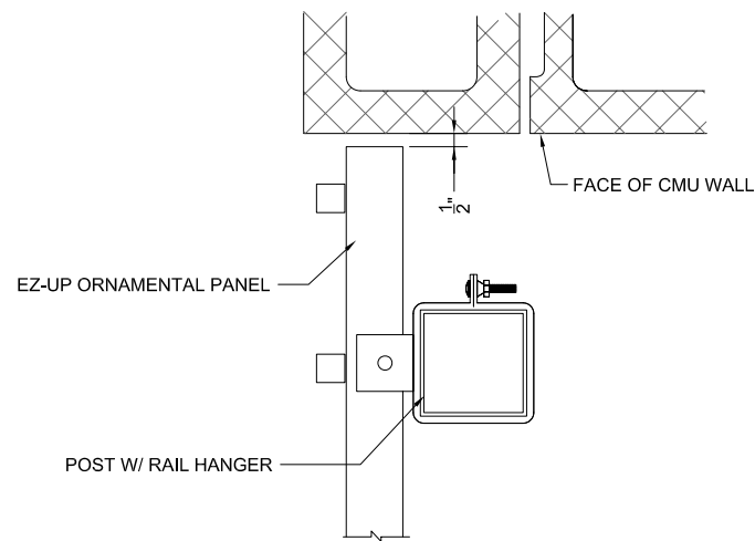
3 FENCE AT WALL DETAIL SCALE: NTS
