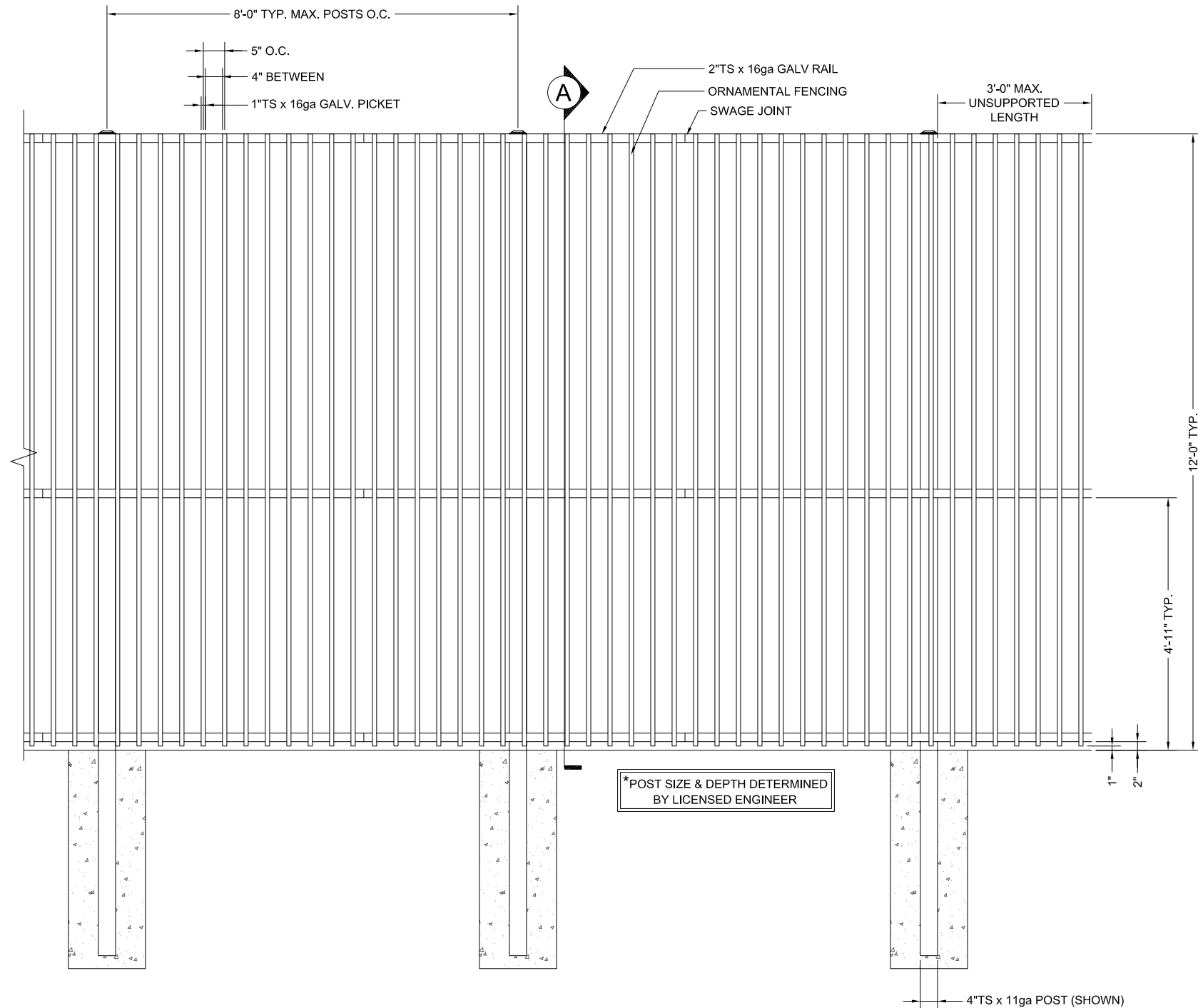
1 EZ-UP ORNAMENTAL ELEVATION SCALE: NTS
