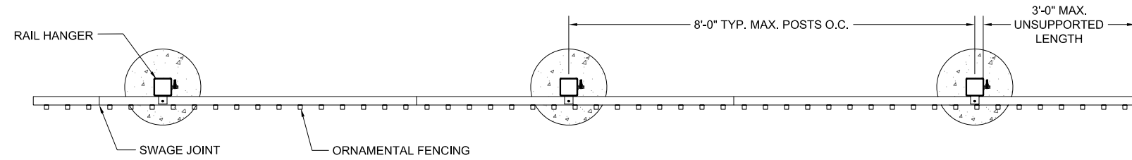
2 EZ-UP ORNAMENTAL PLAN SCALE: NTS
