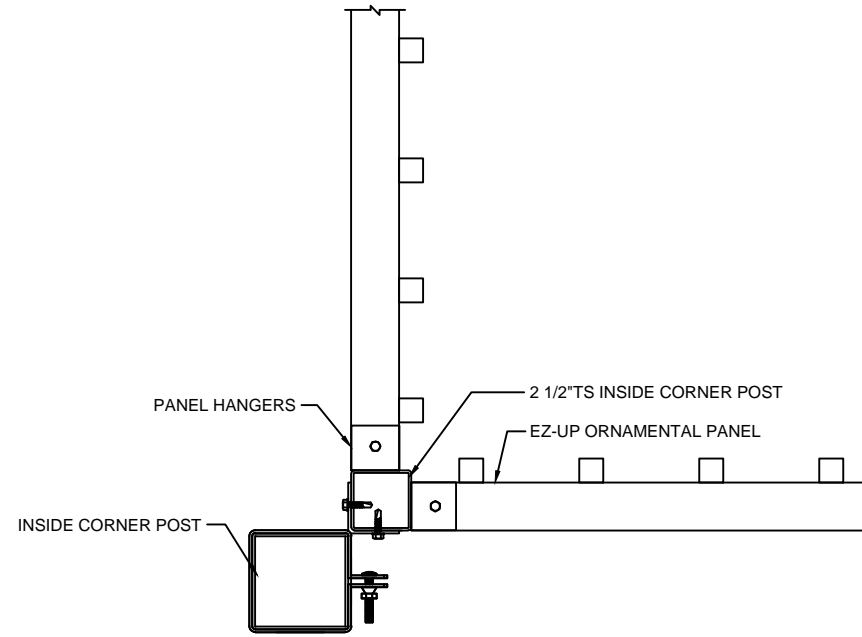
2 INSIDE CORNER DETAIL SCALE: NTS
