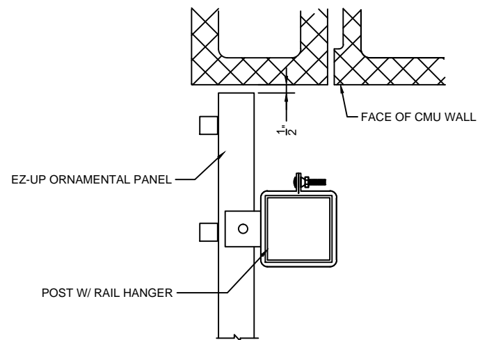
3 FENCE AT WALL DETAIL SCALE: NTS
