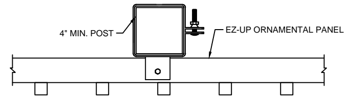
1 LINE POST DETAIL SCALE: NTS
