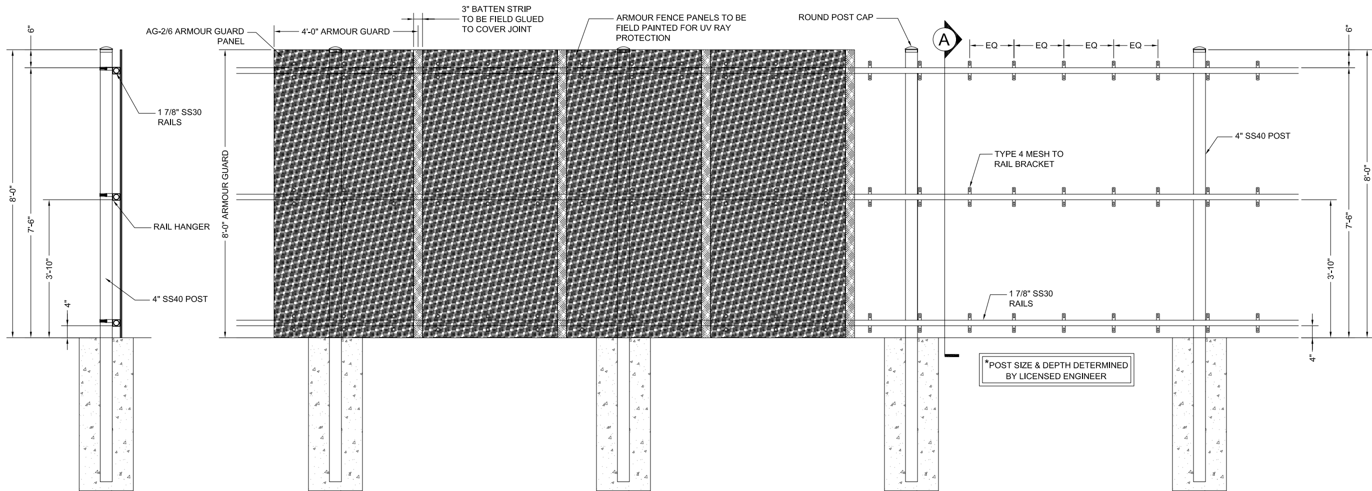
A ARMOR GUARD SECTION SCALE: NTS
