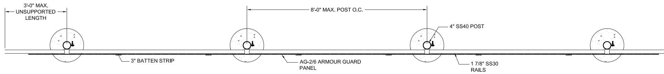
2 ARMOR GUARD PLAN SCALE: NTS
