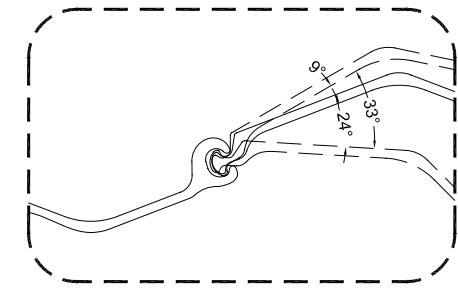
A PANEL ROTATION TOLERANCES SCALE: NTS
