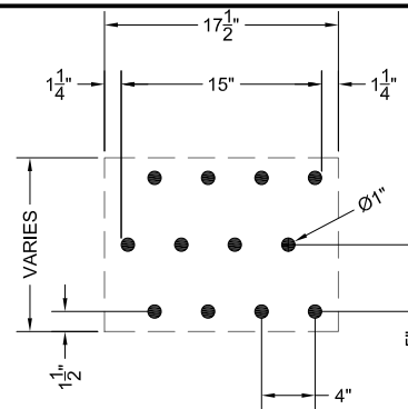
A PANEL ROTATION TOLERANCES SCALE: NTS
